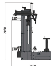
Optional wheel lift.
